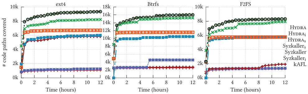
Fig. 16. Code coverage for 12 hours of fuzz testing with kAFL, Syzkaller, HYDRA, and their variants ( i for image-only and s for syscall-only mutation). It indicates that HYDRA aggressively explores the input space that both kAFL and Syzkaller could not reach, and combining both image and input mutators exhibit a synergistic effect in exploring different parts of the input space.
