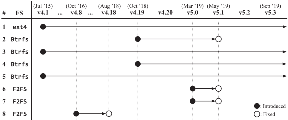
Fig. 19. Lifespan of crash consistency bugs in stable Linux kernel, from v4.1 to v5.3. The black dot (●) denotes the version in which bug is introduced, the white dot (○) marks the version in which bug is fixed, and the arrow (→) refers to the affected versions. Note that the bug ids (#) are consistent with those of Table 6.
