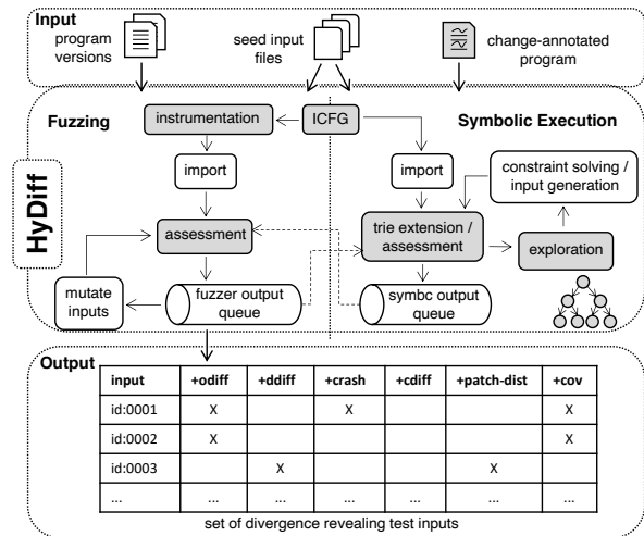
Figure 1: HyDIFF overview.
